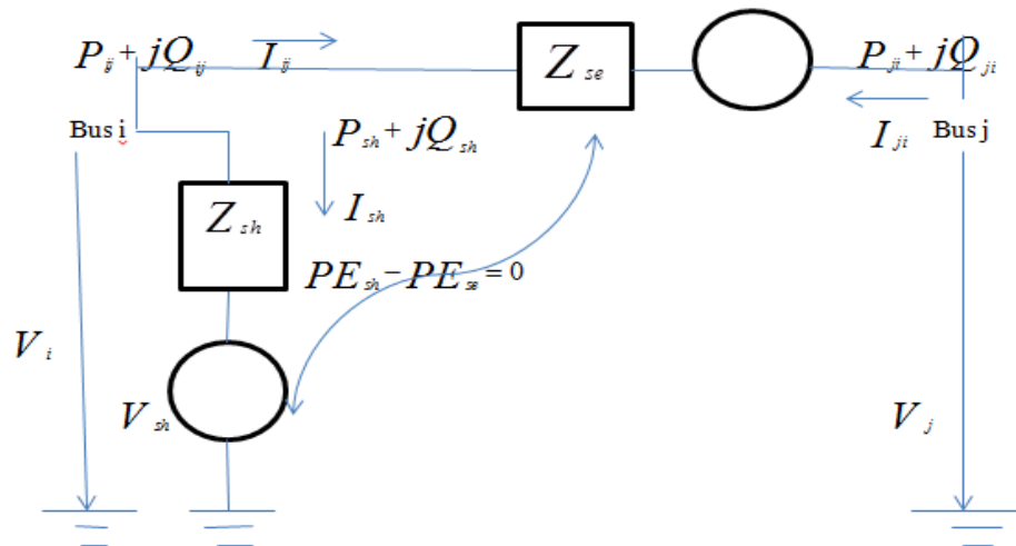
Fig.2 Equivalent circuit of UPFC
