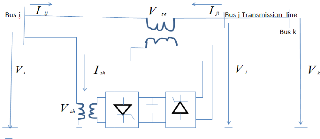
Fig.1 Operating Principle of UPFC
