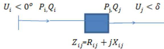
Fig.3 2-Bus Line Model for derivation of Voltage Stability Indices
