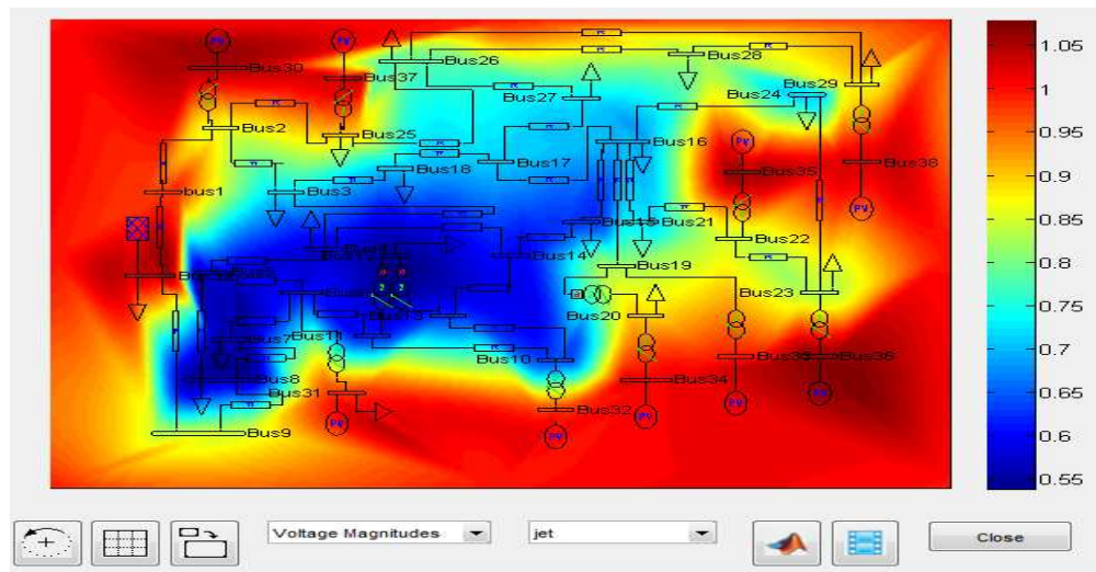
Fig.6 Sparse Matrix Visualization (without UPFC)
