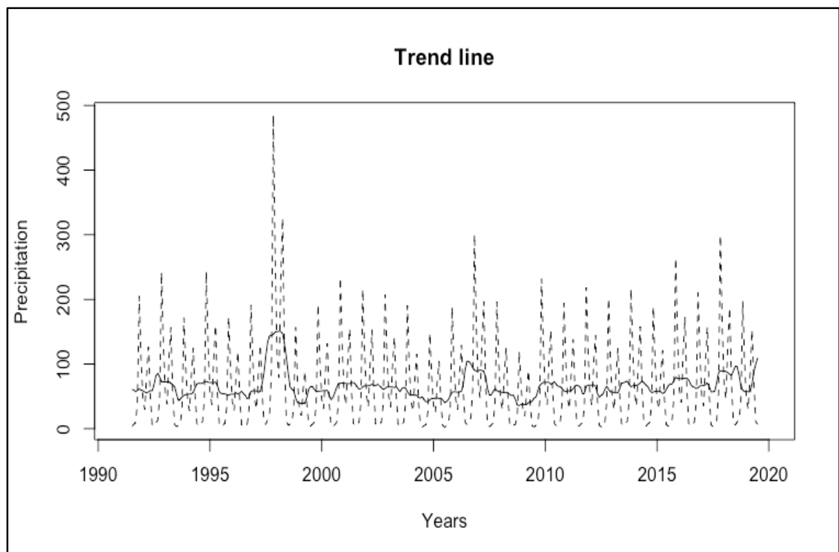
Figure 2: Annual rainfall trend in Makueni County from 1991-2020
