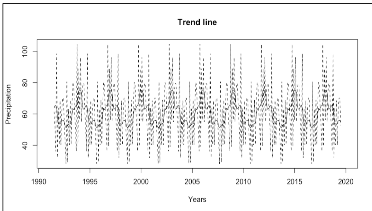
Figure 3: Precipitation Trend for the Short Rain Season (March, April, and May) in Makueni County from 1991 to 2020
