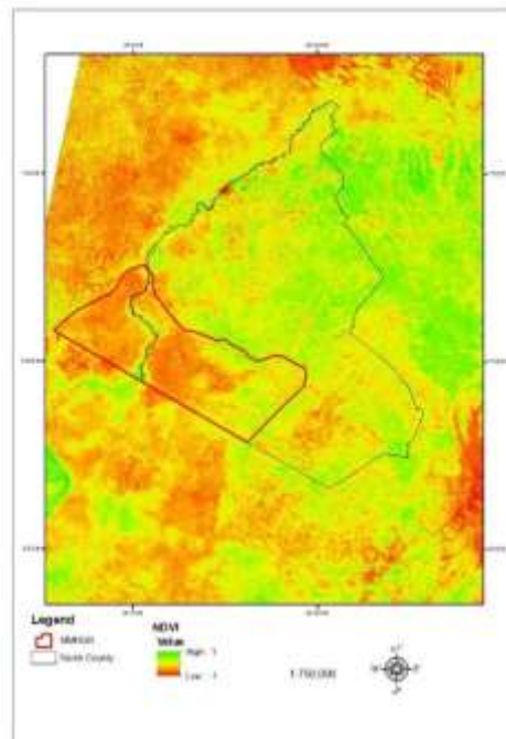
Figure 10. NDVI value for the year 2010 Source: Author (2019)
