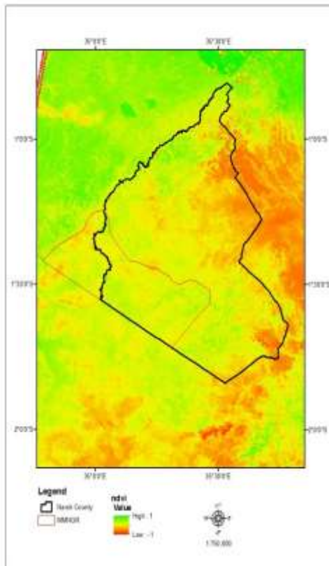
9. NDVI value for the year 2010 Source: Author (2019)
