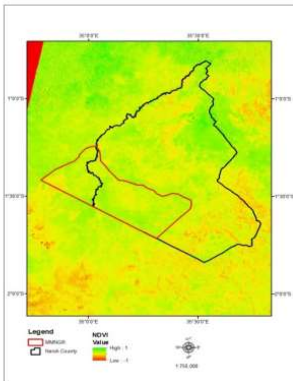
Figure 3. NDVI value for the year 1980 Source: Author (2019)
