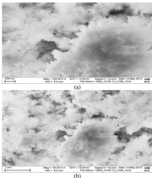
Fig. 8 SEM image of \text{TiO}_2/\text{Nb}_2\text{O}_5 composite thin film on a F: \text{SnO}_2 (a) magnification = 100 K and (b) magnification = 50 K.
