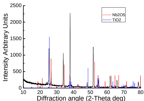
Fig. 9 XRD spectra of \text{TiO}_2/\text{Nb}_2\text{O}_5 composite thin films annealed at 400 °C for 30 min under atmospheric conditions.
