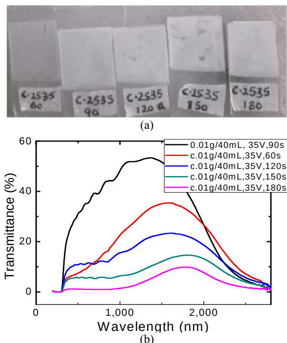
Fig. 2 (a) Photographs and (b) Transmittance spectra for \text{TiO}_2/\text{Nb}_2\text{O}_5 composite electrode thin films electrophoretically deposited from 0.01 g/40 mL, at 35 DCV for varying deposition time.
