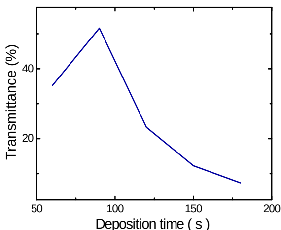
Fig. 3 Variation of transmittance (at 1,508 nm) with deposition time for films electrophoretically deposited at 35 V from 0.01 g/40 mL suspension.
