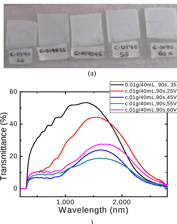
Fig. 6 (a) Photographs and (b) transmittance spectra for \text{TiO}_2/\text{Nb}_2\text{O}_5 composite electrode thin films electrophoretically deposited for 90 s from 0.01 g/40 mL, and for varying voltages.
