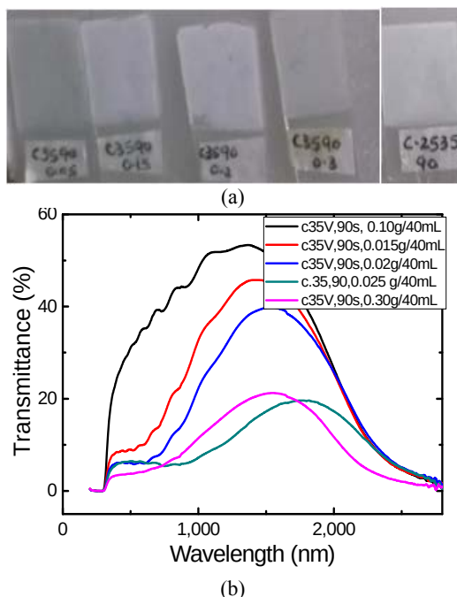
Fig. 4 (a) Photographs and (b) transmittance spectra for \text{TiO}_2/\text{Nb}_2\text{O}_5 composite electrode thin films electrophoretically deposited at 35 DCV for 90 s and from varying powder concentration.
