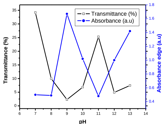
Figure 8. (%) transmittance and absorption edge versus pH values of synthesized ZnO:Al:Ga co-doped nanoparticles with varying pH values
