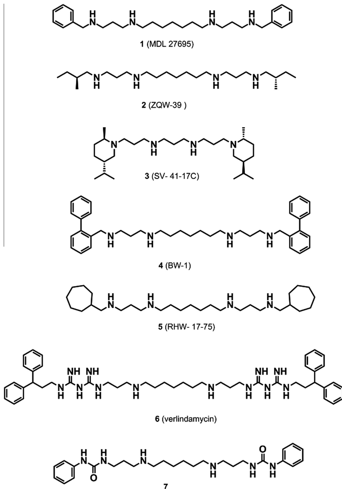
Figure 1. Structures of (bis)alkylpolyamines (compounds 1–5), verlindamycin (compound 6) and 1,14-bis-(phenylurea)-tetradecane (compound 7).
