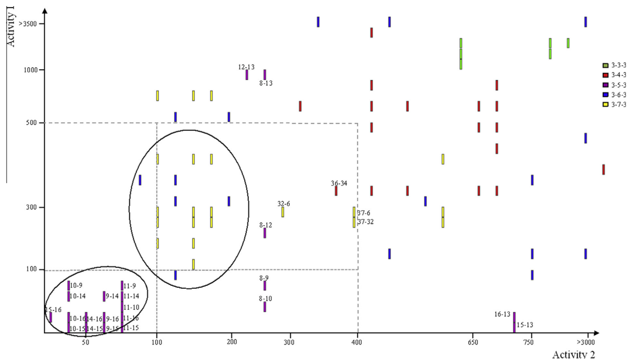
Figure 6. Structure activity landscape analysis for the symmetrically substituted (bis)urea- and (bis)thiourea polyamines. Pairwise activity to structural feature analysis was performed with Activity Cliff Analysis (Osiris DataWarrior V 3.12.1) on the complete series from Figure 5 at a stringency of 80% similarly in structural features. Cluster analysis based on backbone structural features. In all cases, two structurally similar isosteres were compared and a single bar acts as identifier of such correlations based on the respective activities of the two isosteres as indicated on the two axes (decreasing potency from crosspoint). Activity values are based on the In vitro IC 50 values in nM (asexual P. falciparum parasites 3D7). Isostere pairs are identified numerically based on compound numbers in Figure 5 for example, 15–16 with activity 1–activity 2 descriptors.
