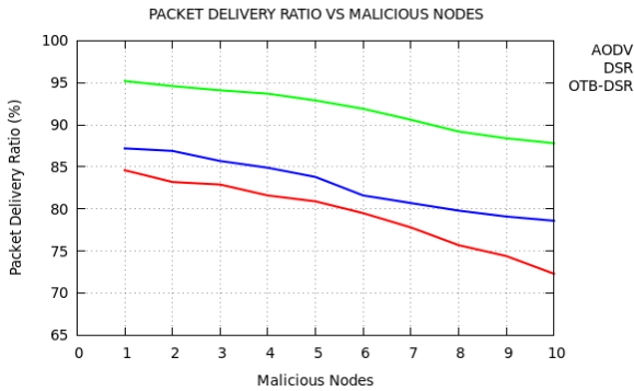
Figure 7. Packet Delivery Ratio versus Malicious Nodes
