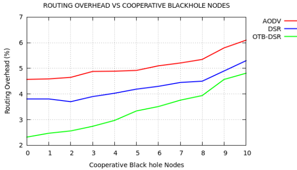
Figure 9. Routing Overhead Versus Cooperative Blackhole Nodes
