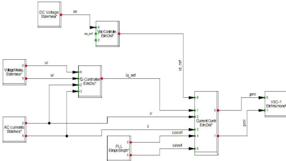
Fig 8.VSC 1 controller set up
