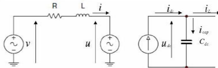
Fig 3. (a) Voltage source for the AC side; (b) Current source for DC side
