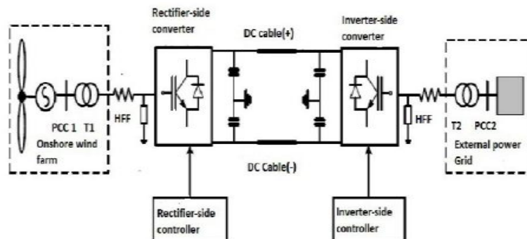
Fig 7. VSC-HVDC with wind farm
