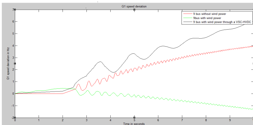
Fig. 15. G1 speed deviation for a fault 2s cleared at 2.45s
