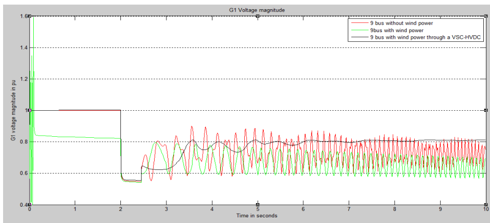
Fig. 13.G1 Voltage magnitude for a fault 2s cleared at 2.45
