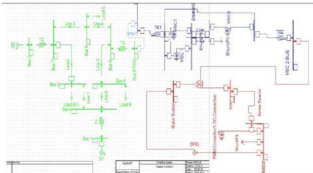
Fig. 10. VSC-HVDC with wind farm connected to 9 bus system
