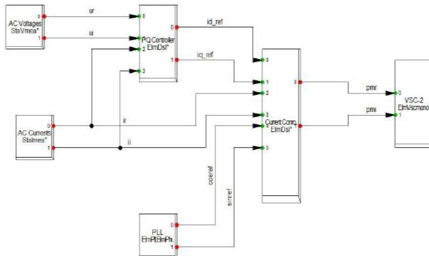
Fig. 9. VSC 2 system control set up
