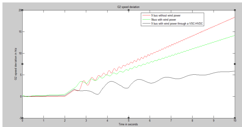
Fig. 16. G2 speed deviation for a fault at 2s cleared at 2.45
