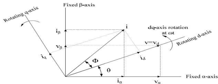
Fig 1. The transformation of axes for vector control
