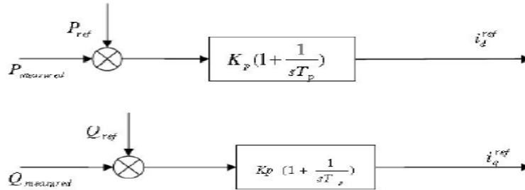
Fig 5. Active and reactive power controllers loop in dq axes
