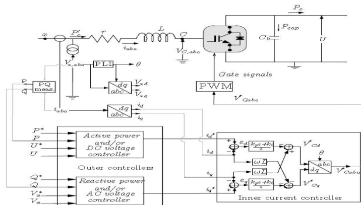
Fig.2. Complete diagram of VSC with inner and outer controller
