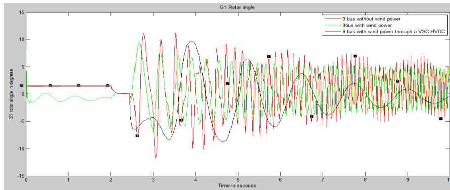
Fig. 11.G1 rotor angle for a fault 2s cleared at 2.45
