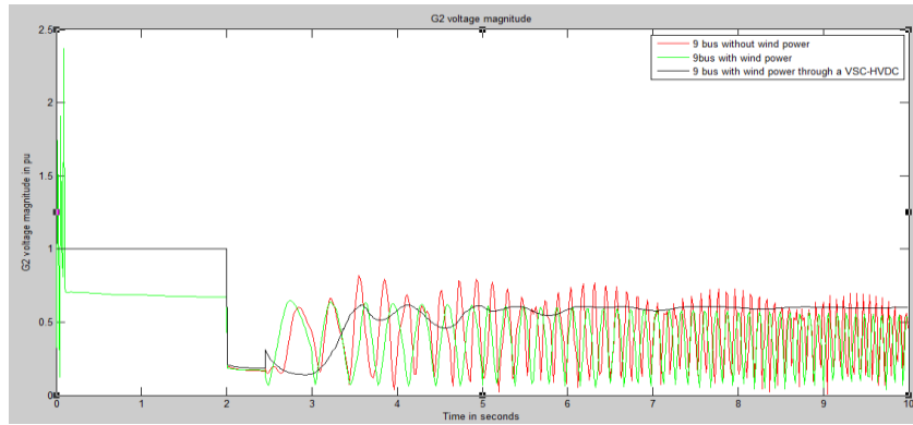
Fig. 14. G2 voltage magnitude for a fault at 2s cleared at 2.45
