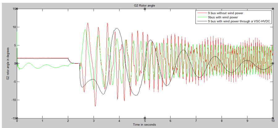
Fig 12. G2 rotor angle for a fault at 2s cleared at 2.45
